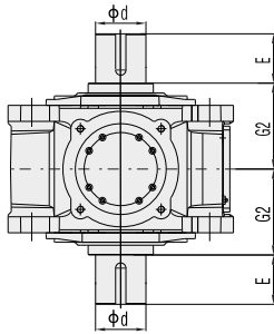
H2..VS Parallel key solid shaft
