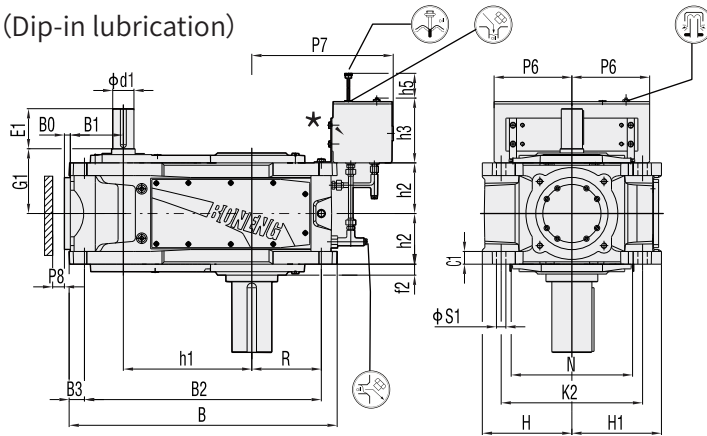
H2..VS Parallel key solid shaft
