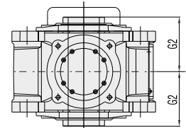
H2..VK Hollow shaft with involute spline
